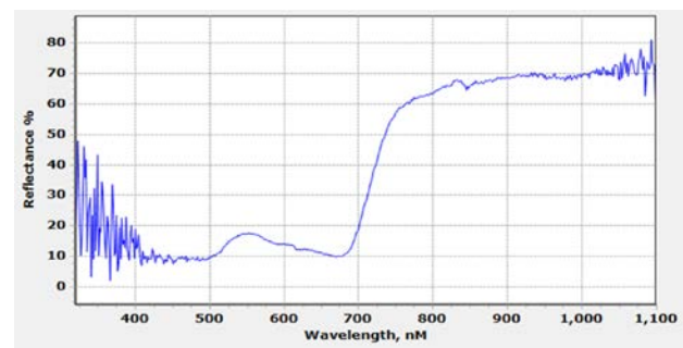
Figure 7. An example of light reflectance signature taken from turfgrass under field conditions.
